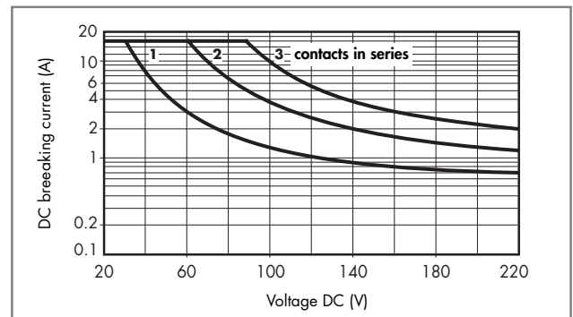
H 62 - Maximum DC1 breaking capacity
