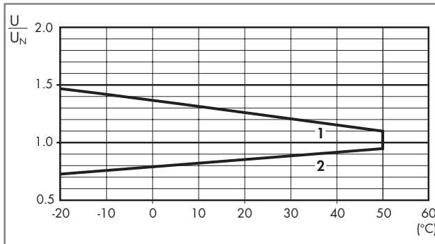
R 62 - DC coil operating range v ambient temperature Normally open contacts
