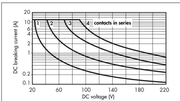
H 56 - Maximum DC1 breaking capacity Changeover version
