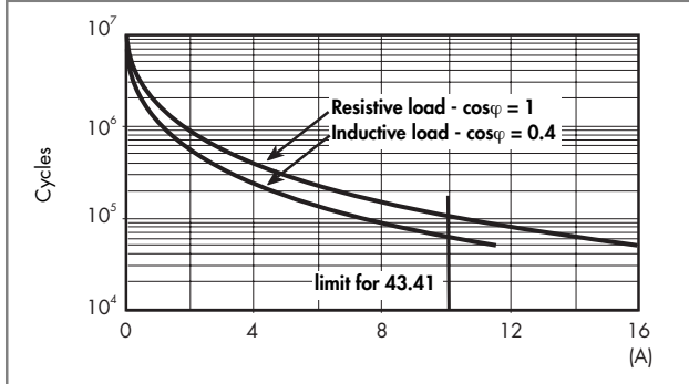
F 43 - Electrical life (AC) v contact current
