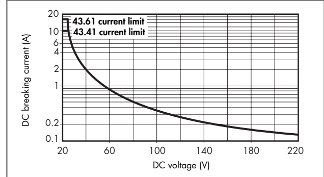
H 43 - Maximum DC1 breaking capacity
