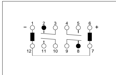
Reset position of 2a2b type
