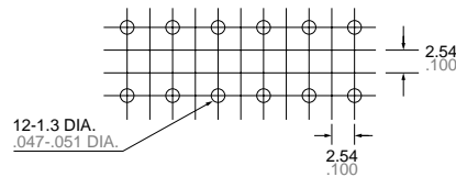
PC board pattern (Copper-side view)
