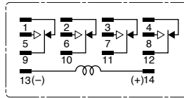
4PDT (RY4/RM42)
