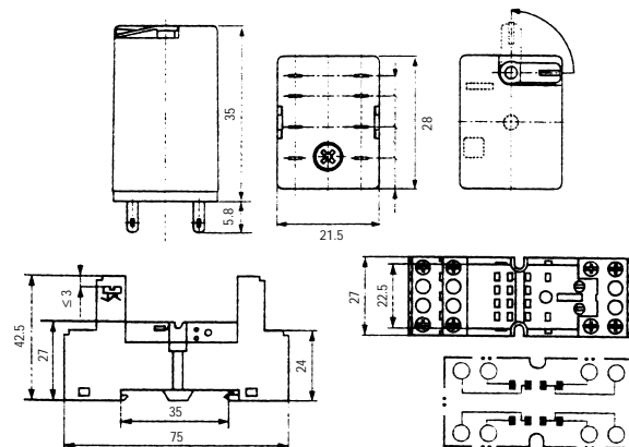
HY21 plug-in version, screw terminals socket SRN2-S
