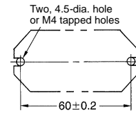
Mounting Holes
