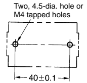
Mounting Holes
