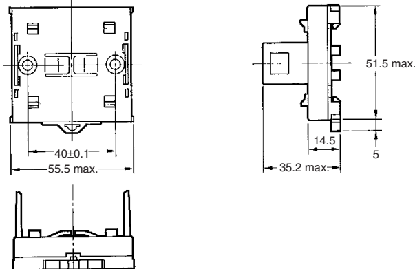
Mounting Holes (Bottom View)
