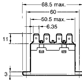
G7L-1A-TUBJ with Test Button
