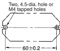
Mounting Holes
