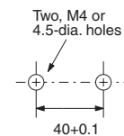
Mounting Holes (Bottom View)
