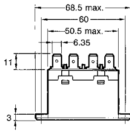
G7L-2A-TUBJ with Test Button
