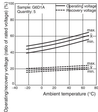
Ambient Temperature vs. Operating/Recovery Voltage G6D-1A-ASI
