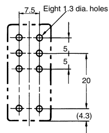
Mounting Holes
