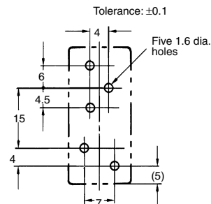
Mounting Holes
