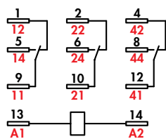
NEMA IEC Wiring Diagram Bottom View
