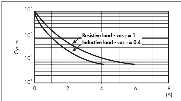
F 34 - Electrical life (AC) v contact current
