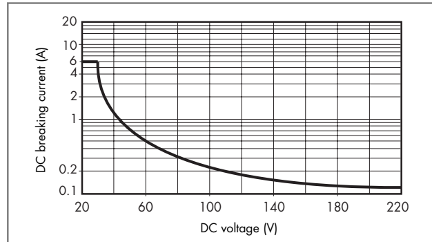
H 34 - Maximum DC1 breaking capacity
