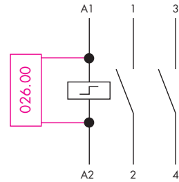
Example of wiring diagram of type 026.00 This module is necessary when using between 1 and a maximum of 15 illuminated push buttons in the coil circuit (Each 1.5 mA max, 230 V AC). It must be connected in parallel to the coil of the relay.
