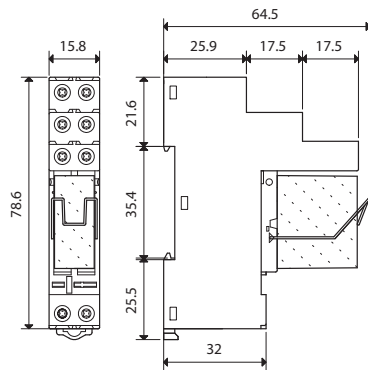
48.12 Screw terminal
