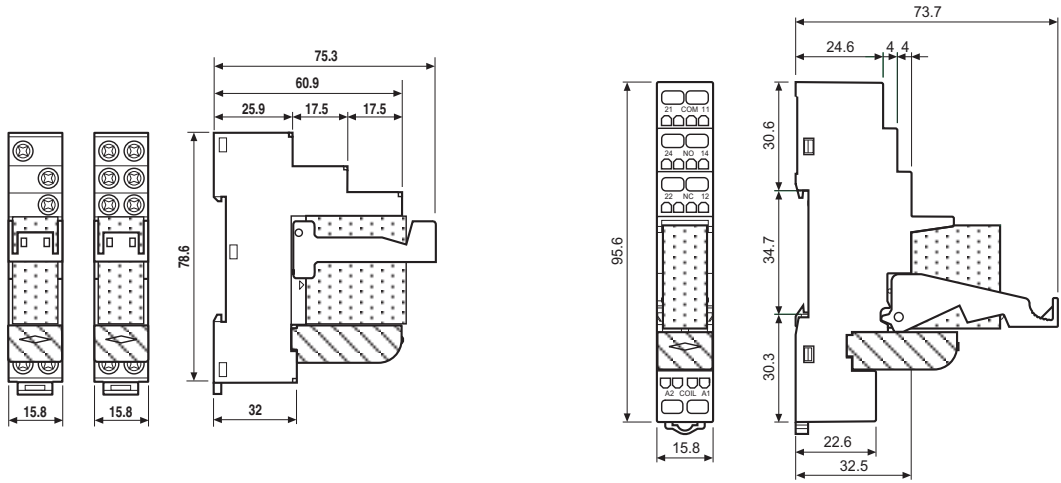
48.31 48.52 / 48.61 / 48.62 Screw terminal
