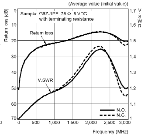
High-frequency Characteristics at 75 Ω (Return Loss, V.SWR)
