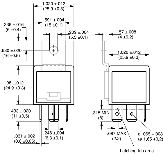
Quick connect terminal similar to ISO 8092-1
