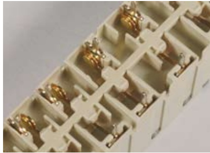
Set of contacts with actuator
