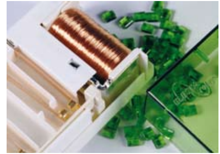
Open relay
