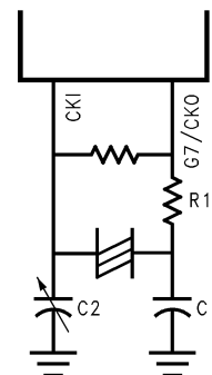
Without On-Chip Bias Resistor
