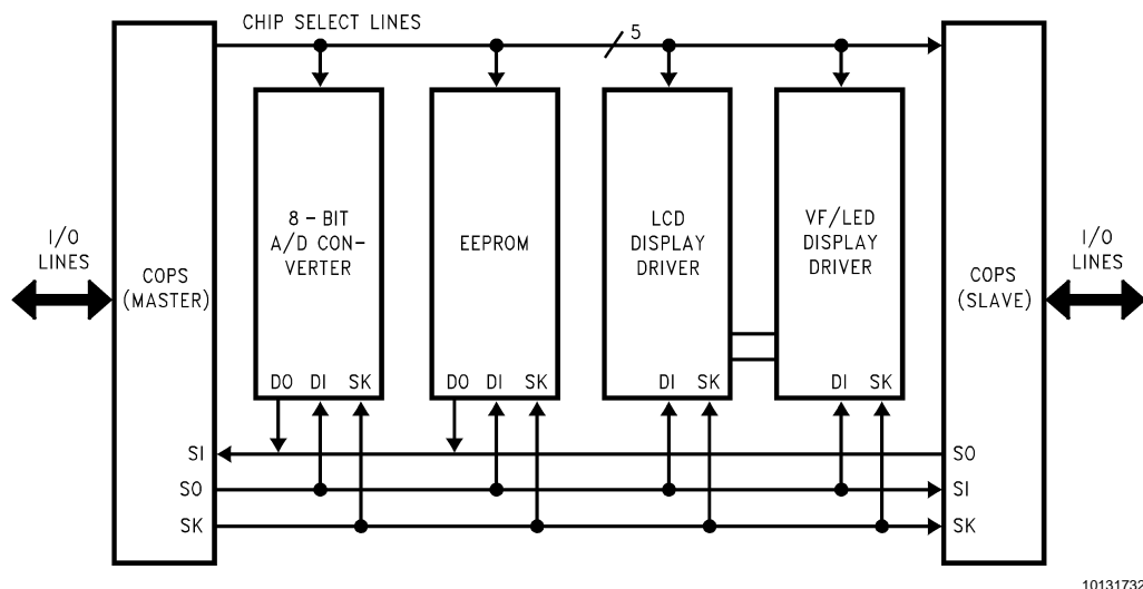
FIGURE 28. MICROWIRE/PLUS Application
