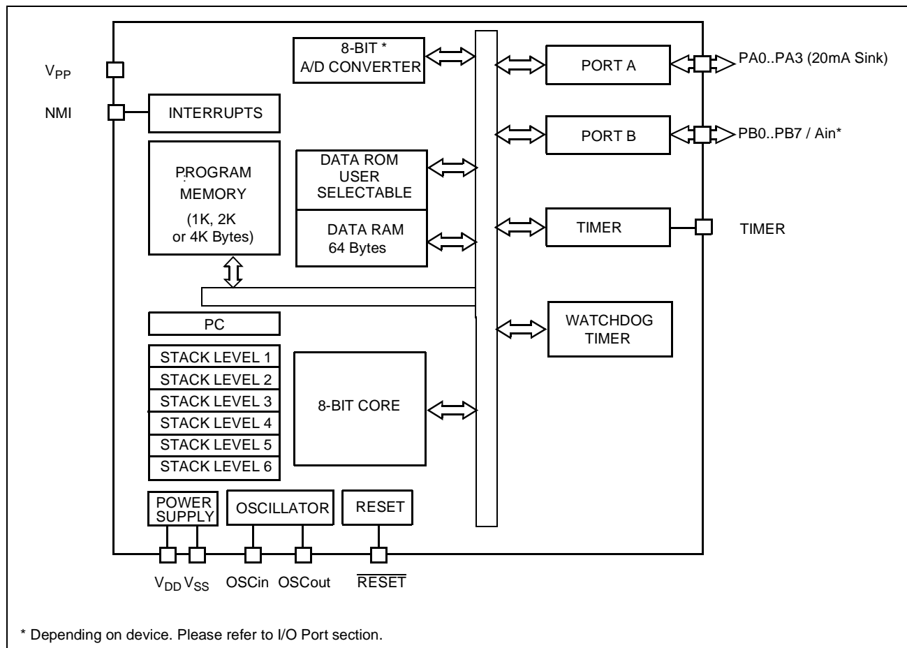
Figure 1. Block Diagram
