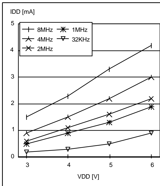
Figure 42. Typical I_{DD} in RUN vs. f_{CPU}
