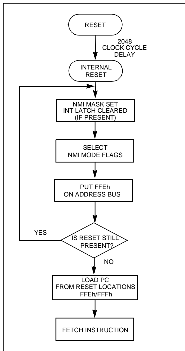
Figure 16. Reset Processing
