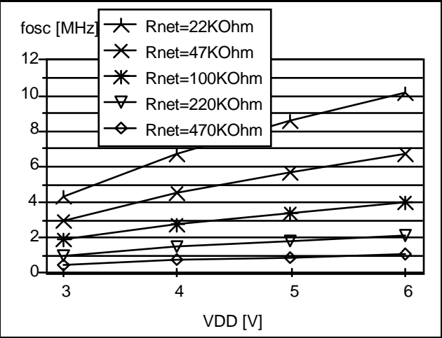
Figure 52. Typical RC Oscillator frequency vs. V_{DD}
