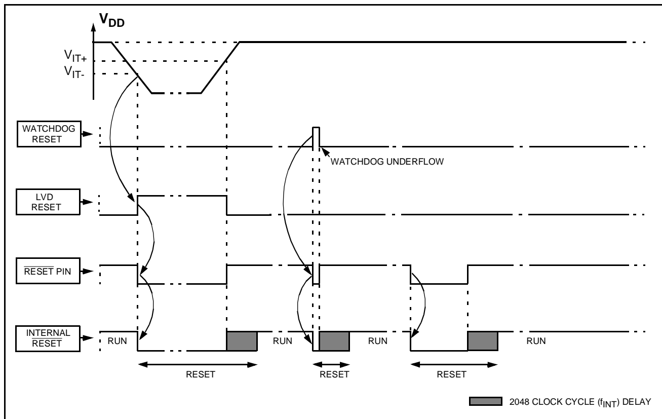
Figure 13. RESET Sequence
