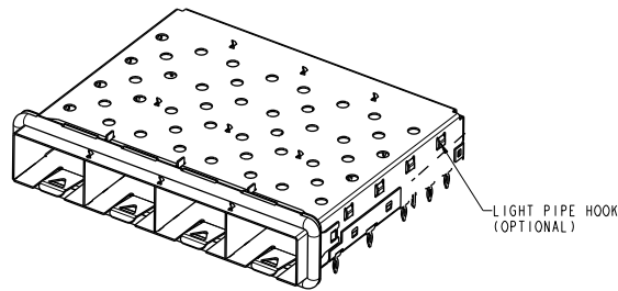
SFP PLUS 1X4 CAGE ASSEMBLY
