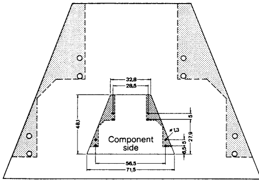
Printed Circuit Board for Component Housings with Screw Connection
