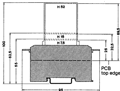
Dimensional drawing of electronic module EMG
