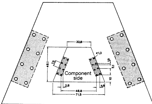
Printed Circuit Board for Component Housings with Tab Connection
