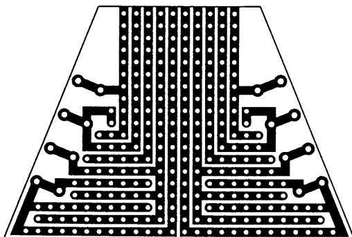
Printed Circuit Board P1-UEG-FS/FS
