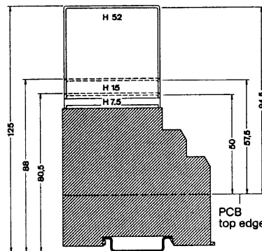
Dimensional drawing of electronic module EME
