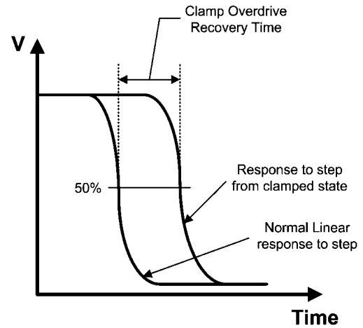
FIGURE 7. Clamp Overdrive Recovery Time
