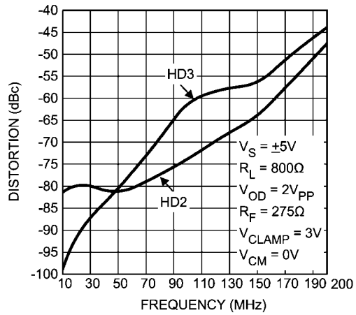
Distortion vs. Frequency Single-Ended Input
