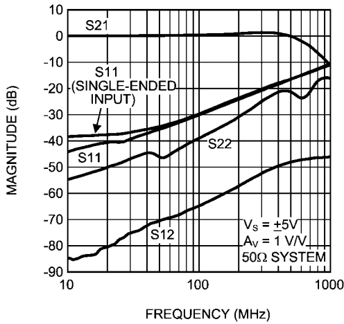
Differential S-Parameter Magnitude vs. Frequency
