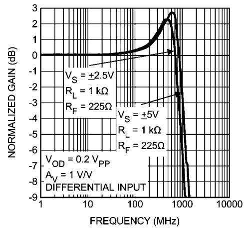
Frequency Response vs. Supply Voltage with R_L = 1 k\Omega
