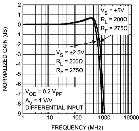
Frequency Response vs. Supply Voltage with R_L = 200\Omega
