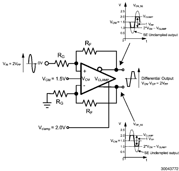
FIGURE 6. Clamp Operation
