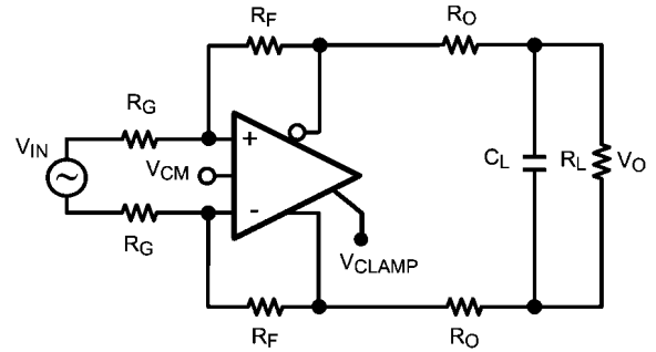
FIGURE 1. Typical Application
