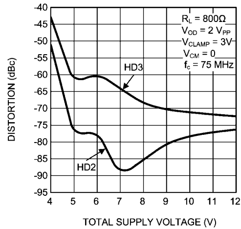
Distortion vs. Supply Voltage
