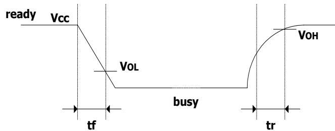
Figure 34. Ready/Busy AC Waveform
