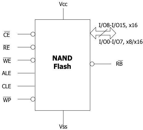
Figure 1: Logic Diagram
