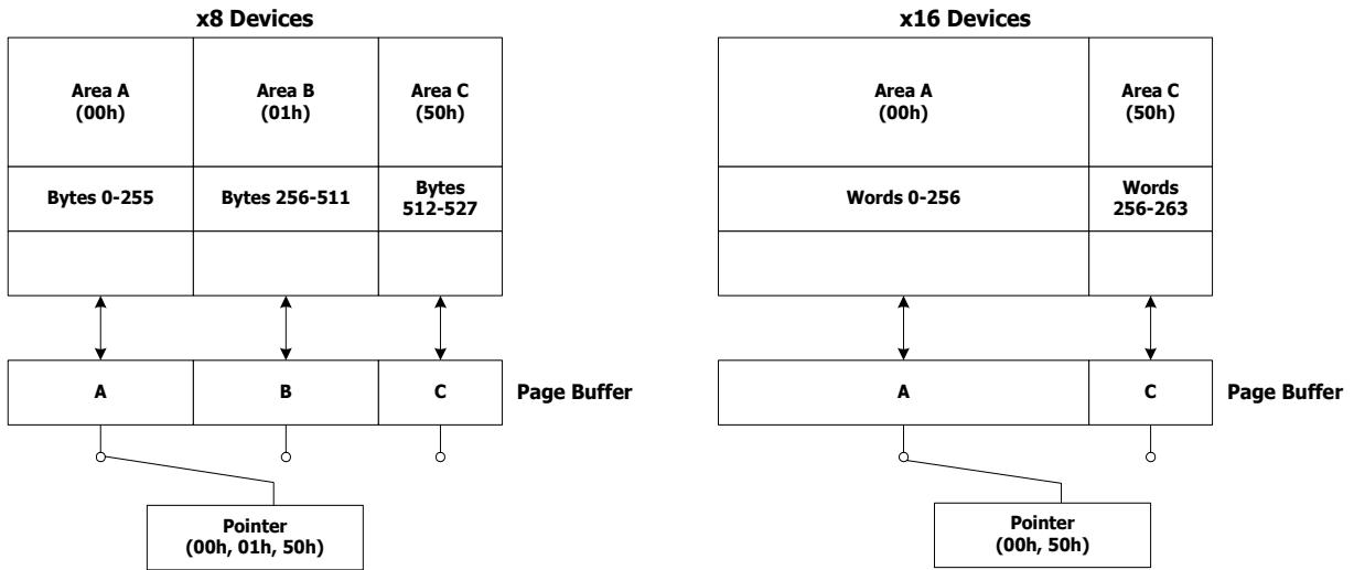
Figure 8. Pointer Operation
