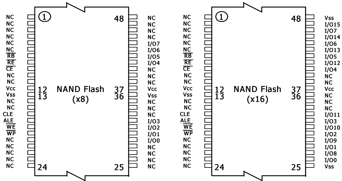
Figure 3. 48-TSOP1 Contactions, x8 and x16 Device
