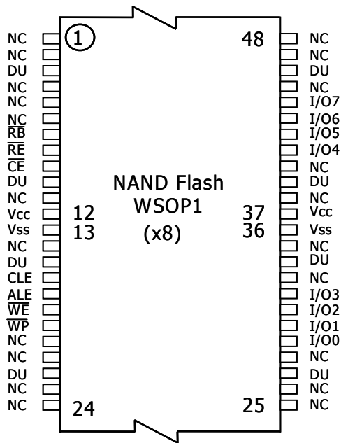
Figure 4. 48-WSOP1 Contactions, x8 Device
