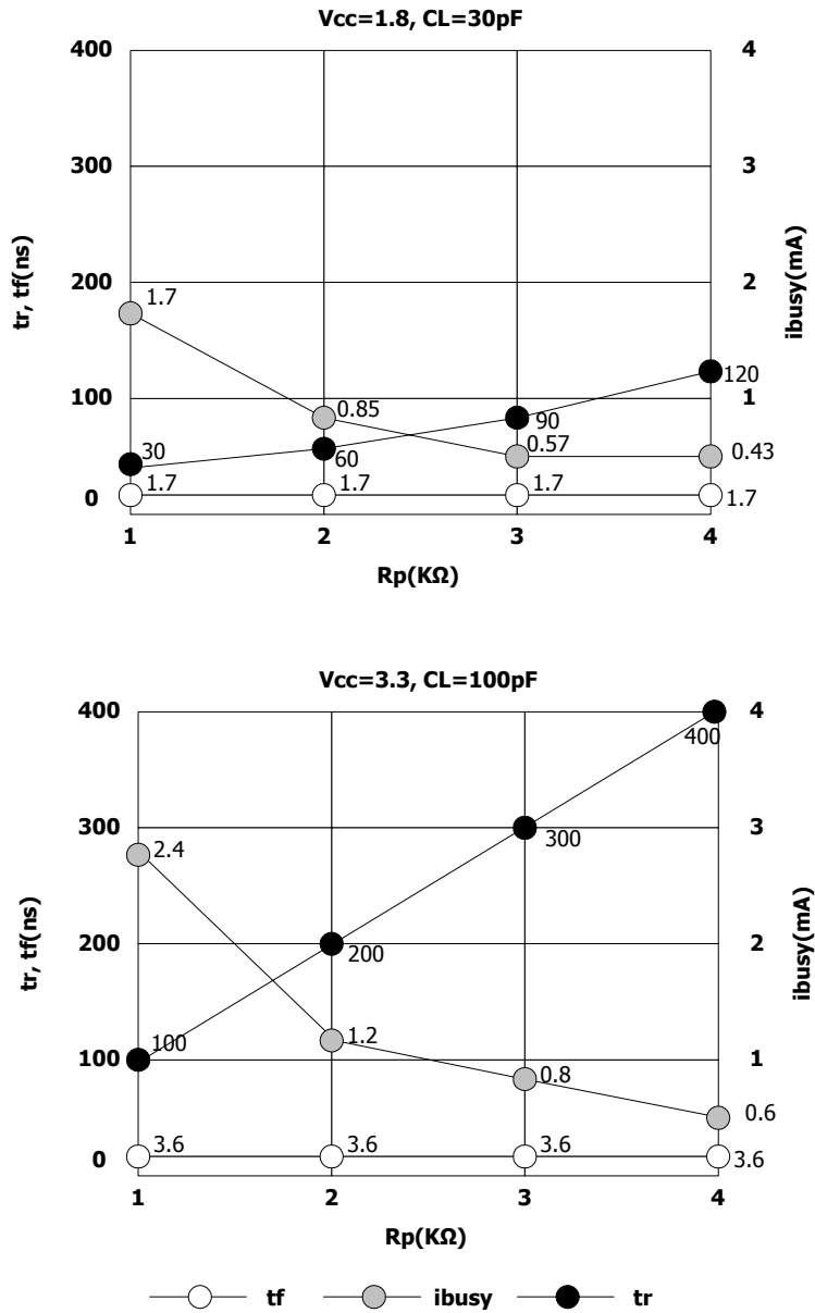
Figure 36. Resistor Value Waveform Timings for Ready/Busy Signal
