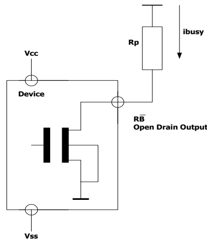
Figure 35. Ready/Busy Load Circuit
