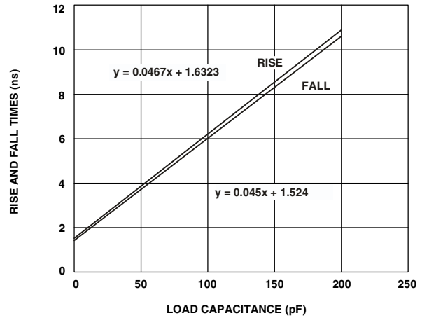
Figure 38. Typical Output Rise/Fall Time (20% to 80%, V_{DDEXT} = Max )
