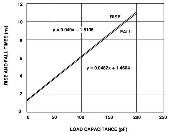
Figure 39. Typical Output Rise/Fall Time (20% to 80%, V_{DDEXT} = Min )
