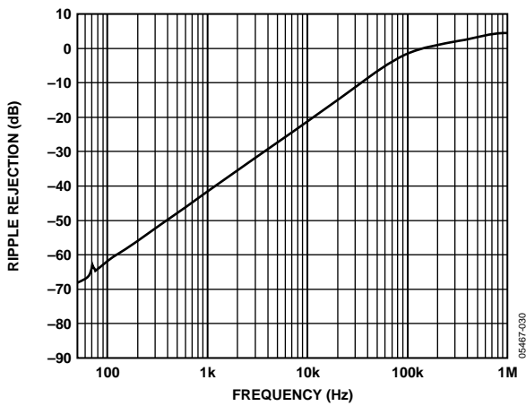
Figure 22. Ripple Rejection Ratio
