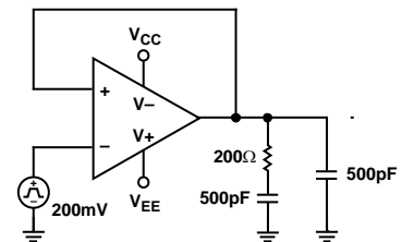
Figure 38. Snubber Network
