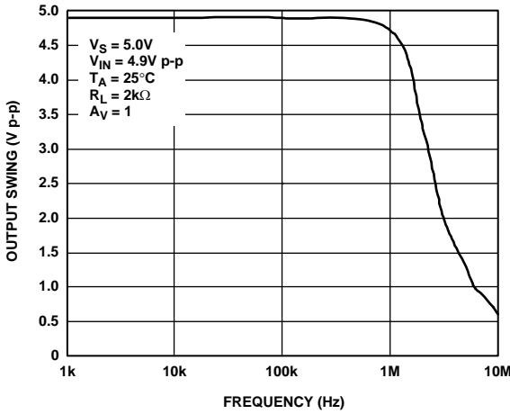
Figure 13. Closed-Loop Output Voltage Swing
