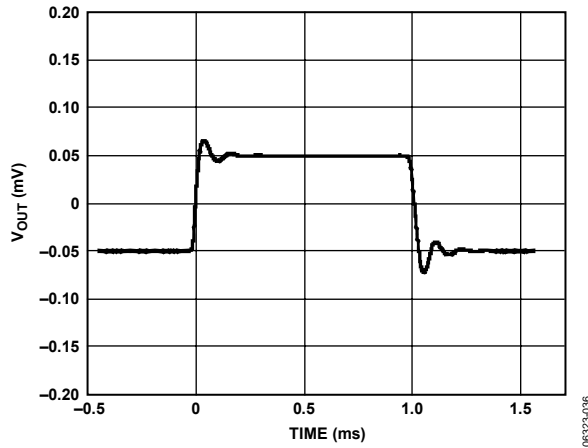
Figure 37. Small Signal Transient Response (100 pF Load Capacitance), V_S = 1.8\text{ V}
