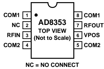
Figure 2. Pin Configuration
