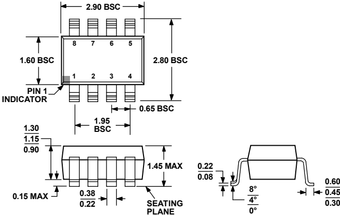
COMPLIANT TO JEDEC STANDARDS MO-178-BA Figure 29. 8-Lead Small Outline Transistor Package [SOT-23] (RJ-8) Dimensions shown in millimeters
