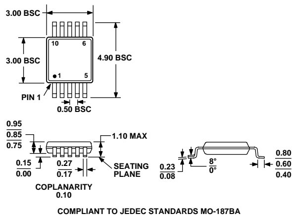
Figure 47. 10-Lead Mini Small Outline Package [MSOP] (RM-10)
