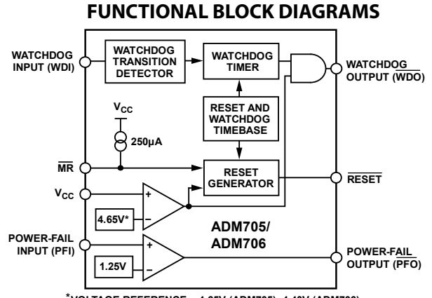
* VOLTAGE REFERENCE = 4.65V (ADM705), 4.40V (ADM706)
