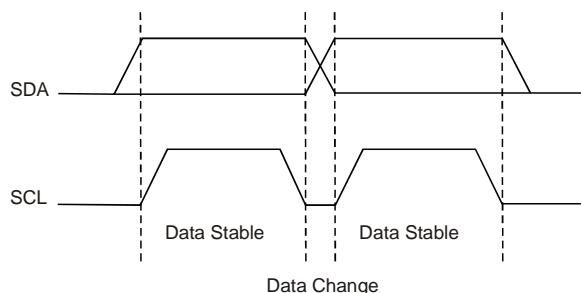
Figure 5.2 Data Transfer
