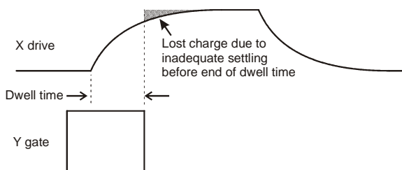
Figure 2.4 X-Drive Pulse Roll-off and Dwell Time
