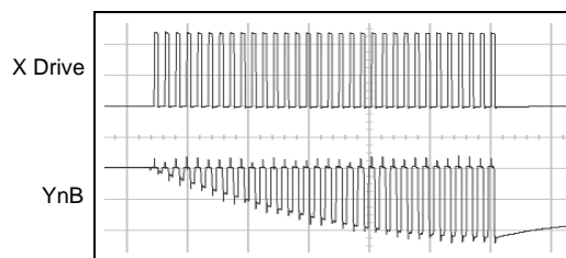
Figure 2.2 VCs - Poor Gain, Nonlinear During Burst
