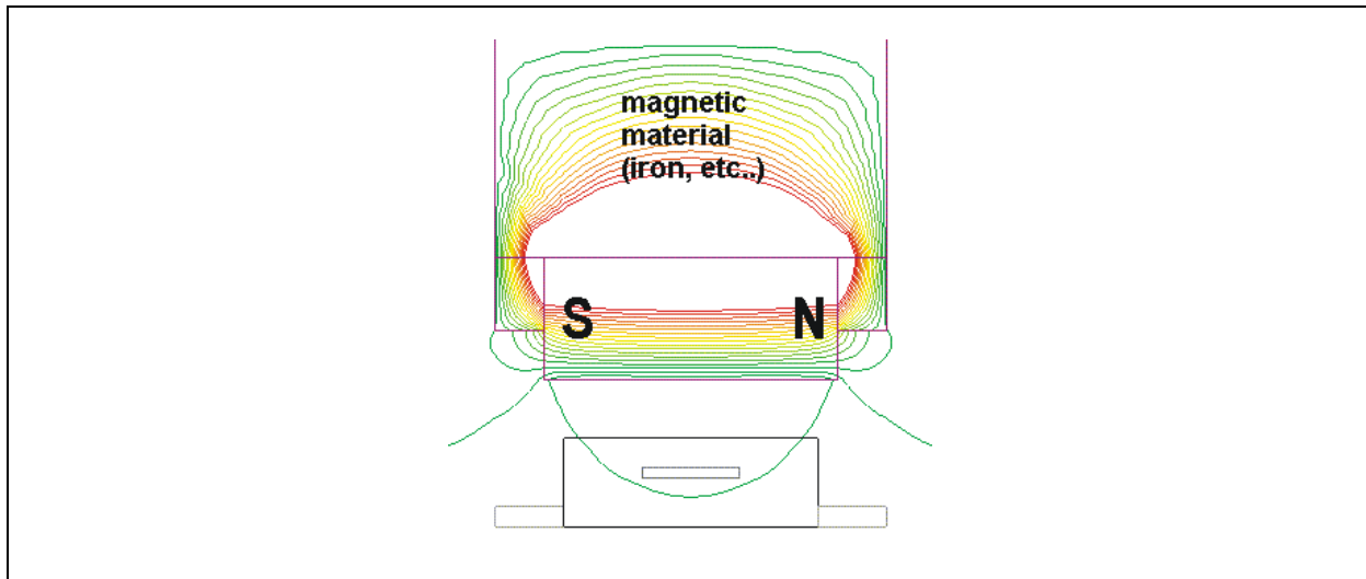
Figure 25. Magnetic Field Lines in Iron Shaft
