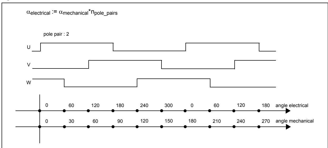
Figure 11. Commutation Mode
