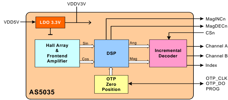
Figure 3: AS5035 Block diagram
