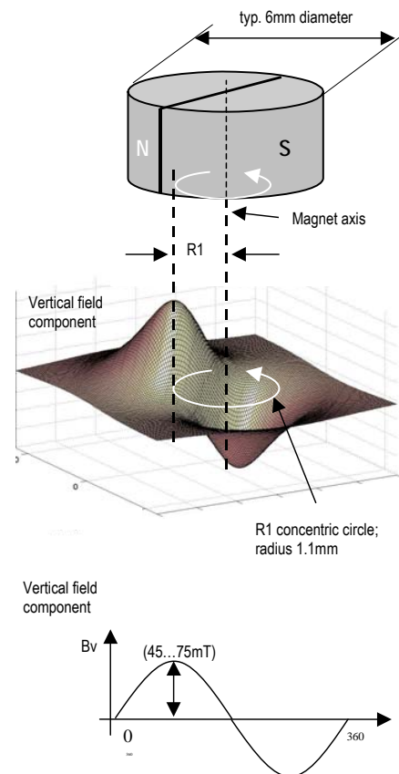
Figure 10: Typical magnet and magnetic field distribution
