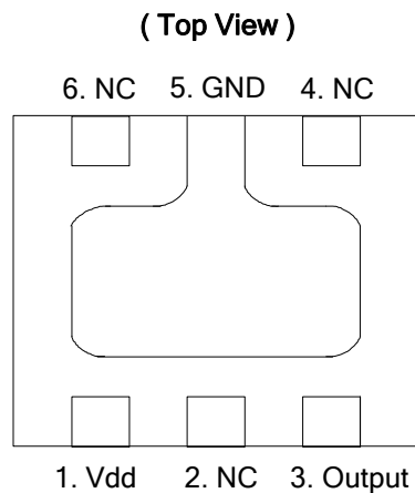
(2) DFN2020-6
