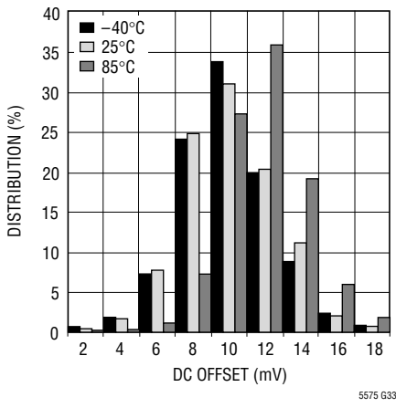
I-Output DC Offset Voltage Distribution vs Temperature
