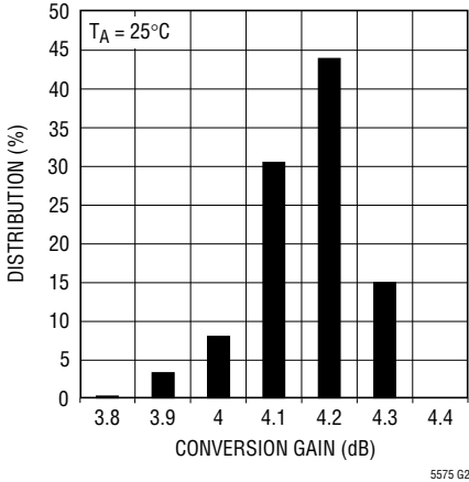
Conversion Gain Distribution at 1900MHz
