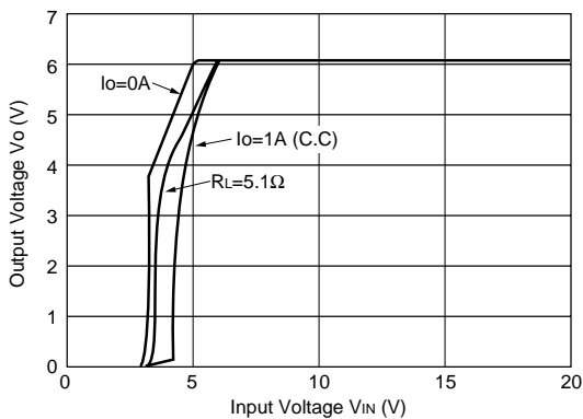
Rise Characteristics
