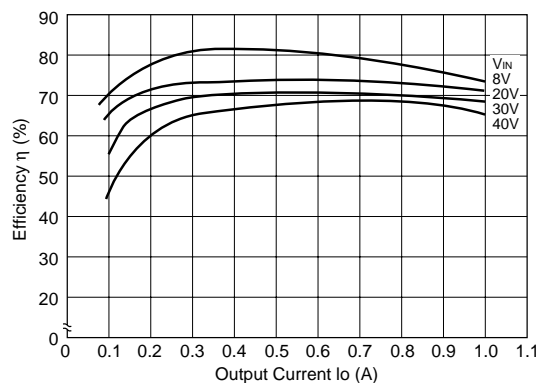
Efficiency Characteristics
