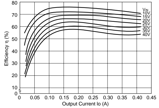
Efficiency Characteristics
