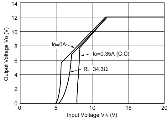
Rise Characteristics
