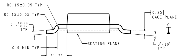
3-Lead SOT-223 Package NS Package Number MP04A
