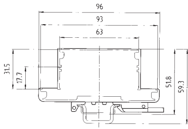
Dimensions for WEB empty housing for sizes 1, 3, 6 and 8 with foot TS 35
