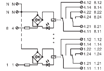
WR4/8-230-2W 250 V 4 A
