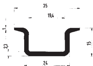
Mounting rail 35 x 15 accord. to DIN EN 60715
