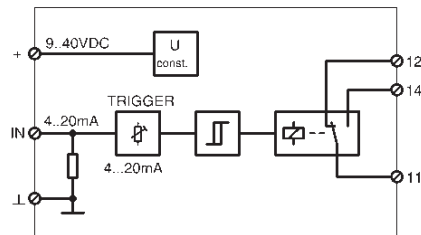
Wiring diagram Current relay SR 4...20 mA
