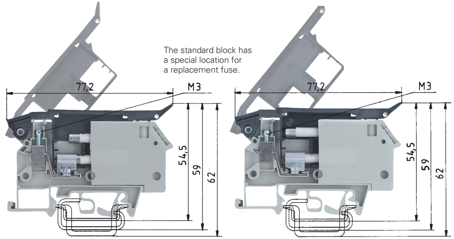
for 5 mm fuses
