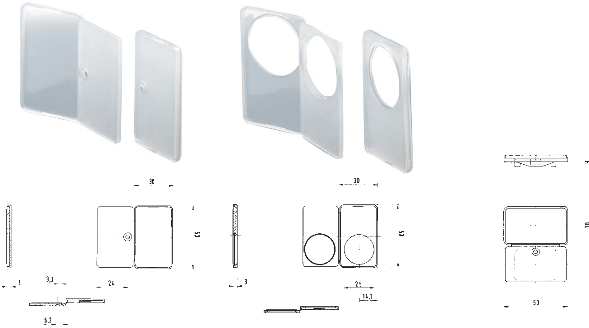
Marking tag
