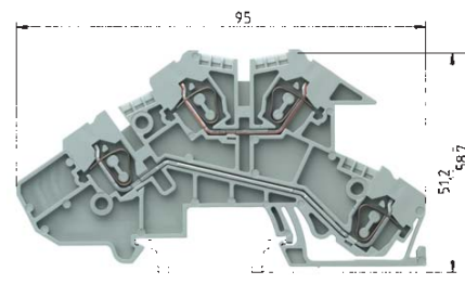
D – line feedthrough D – line feedthrough
