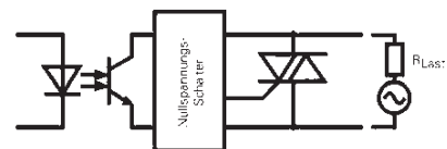
Block diagram of AC output
