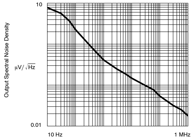
Noise Spectrum
