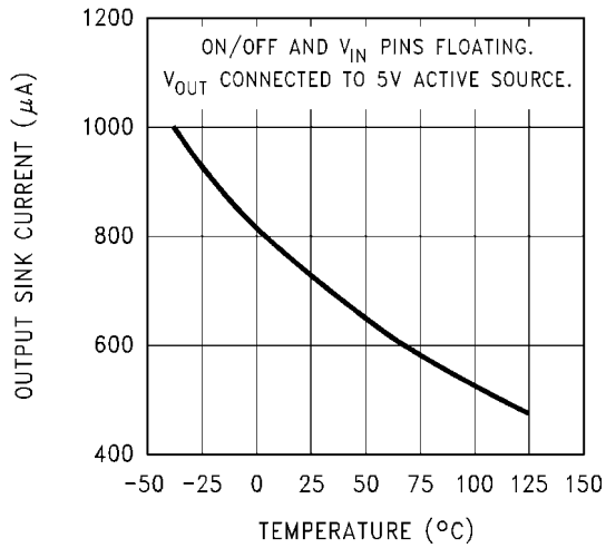
Output Reverse Leakage vs Temperature
