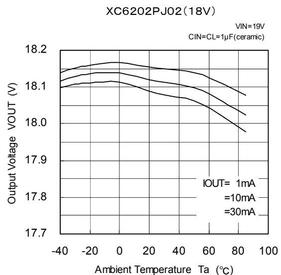
(5) Output Voltage vs. Ambient Temperature
