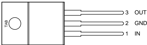
MIC39300-x.xBT TO-220-3 (T)
