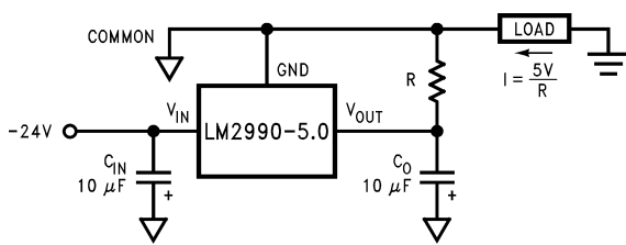
Fixed Current Sink
