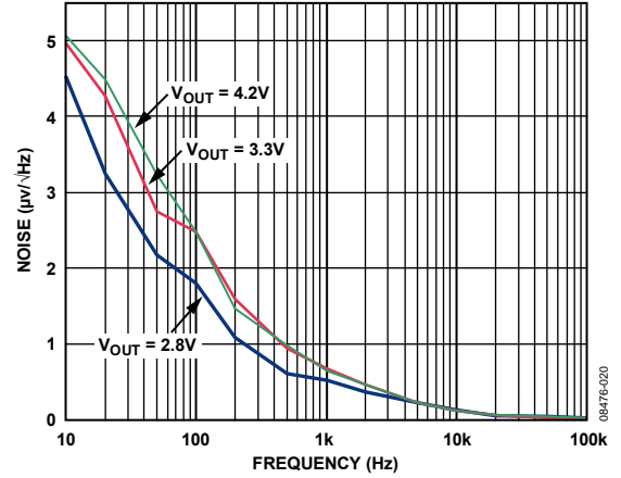
Figure 20. Output Noise Spectrum, V_{IN} = 5V
