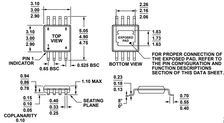
Figure 43. 8-Lead Mini Small Outline Package with Exposed Pad [MINI_SO_EP] (RH-8-1)
