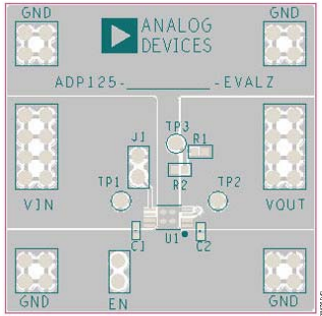
Figure 42. Example ADP125 PCB Layout
