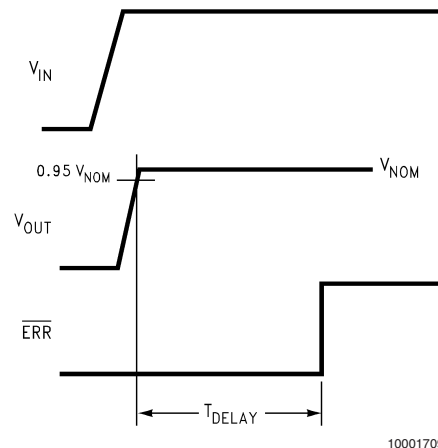
Timing Diagram for Power-Up
