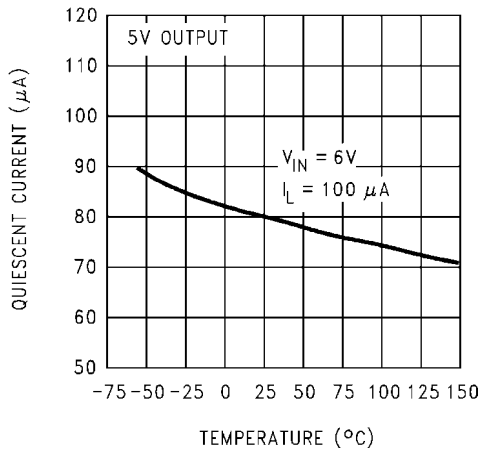
Quiescent Current
