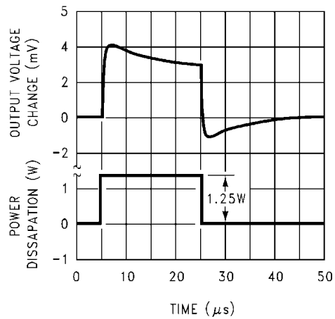
Thermal Response
