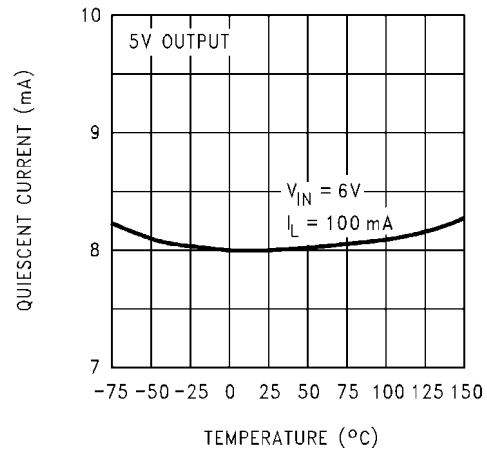
Quiescent Current
