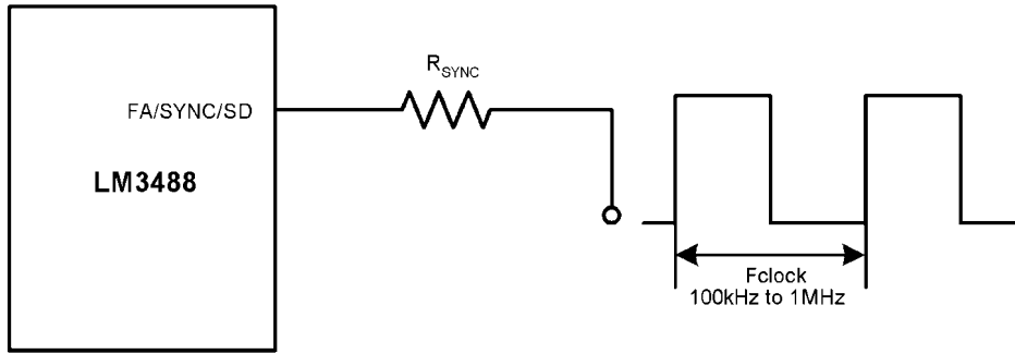
FIGURE 7. Frequency Synchronization
