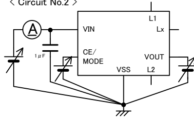
< Circuit No.2 >
