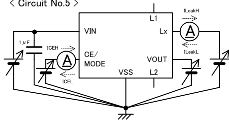
< Circuit No.5 >
