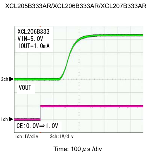
(12) Rise Wave Form
