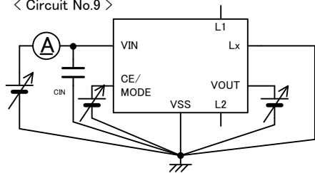
< Circuit No.9 >
