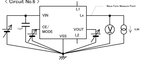
< Circuit No.6 >
