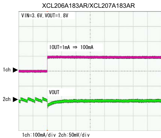
(15) Load Transient Response
