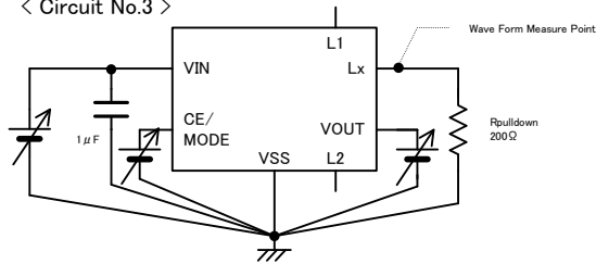
< Circuit No.3 >
