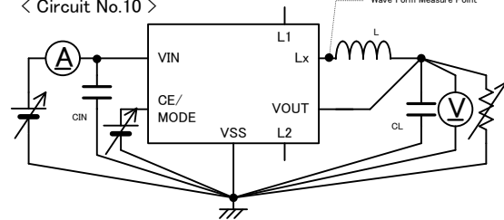
< Circuit No.10 >
